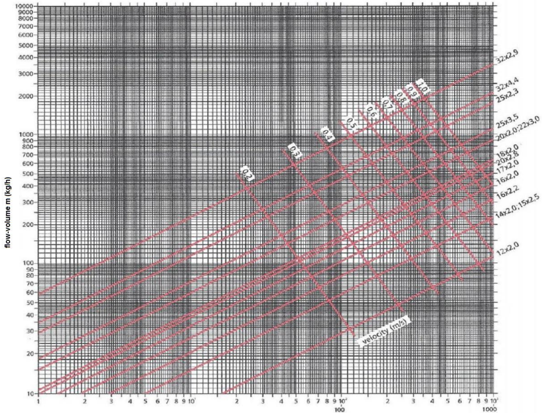
Drukverlies-diagram U-Tube Systems : PE-RT buis
